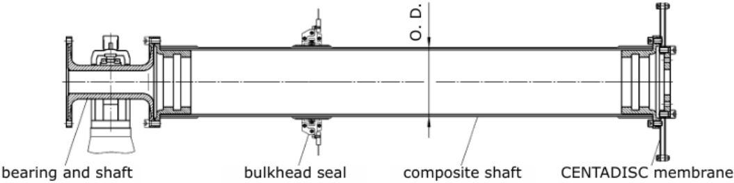
Figure 1: Sectional layout drawing of CENTA Type S high-speed/long span composite shaft assembly, detailed with metallic flange endpoints, bulkhead seal, and bearing interfaces.
